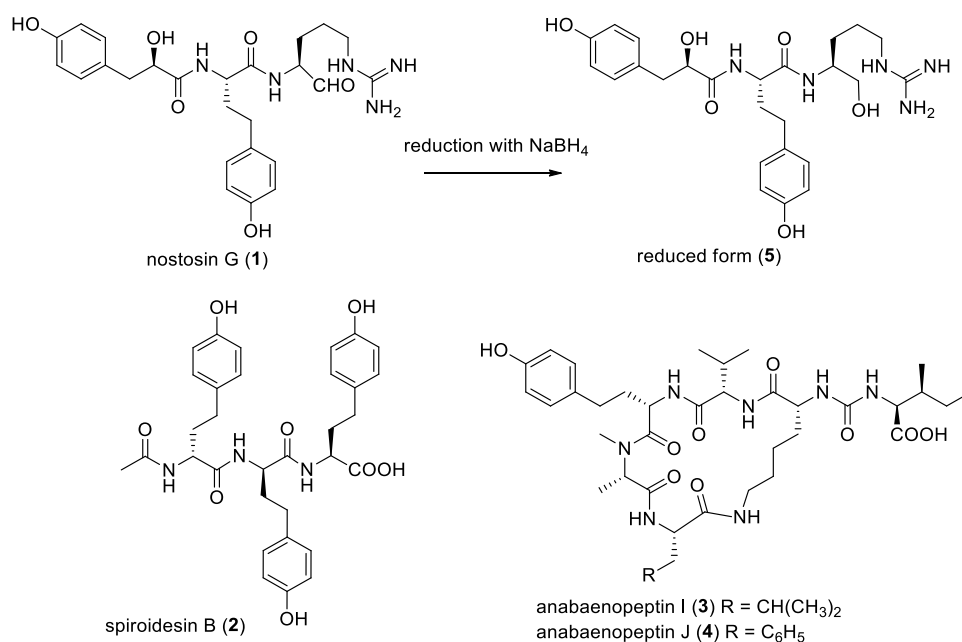
Figure 1. Structures of 1–5 and chemical reduction of 1.
